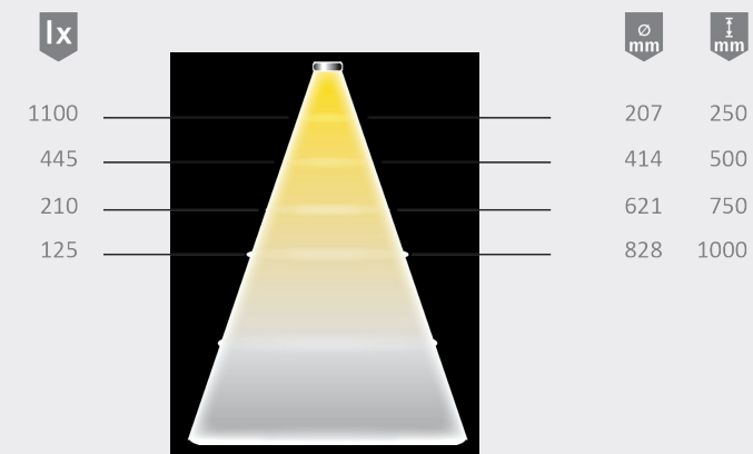
Light distribution diagram 45° - measured in black room
