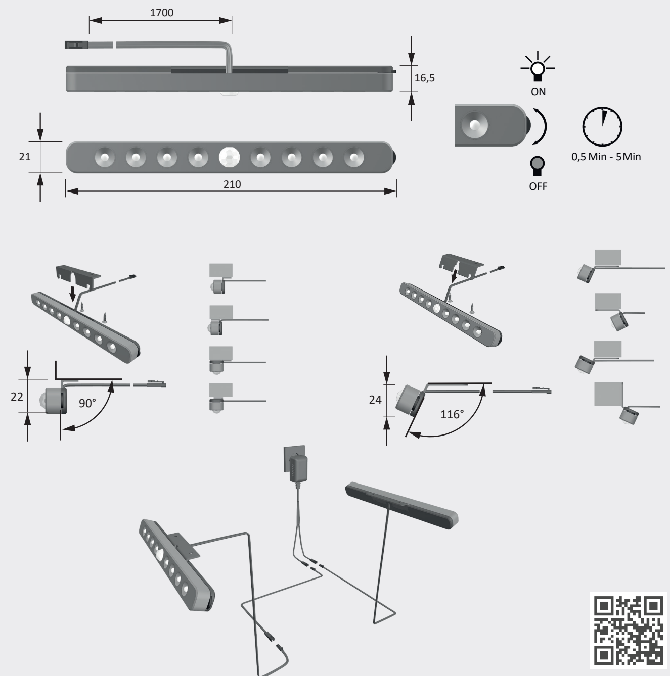
Assembly drawing
