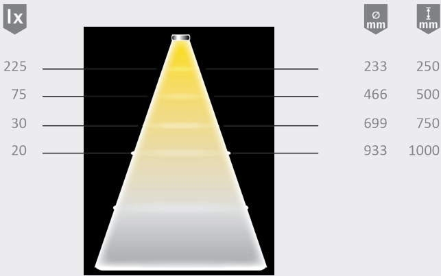
Light distribution diagram 50° - measured in black room
