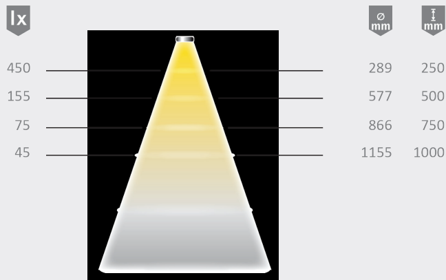
Light distribution diagram 60° - measured in black room
